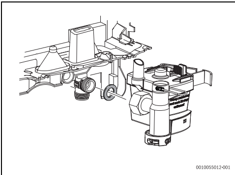
Fig. 28 Additional bushing
