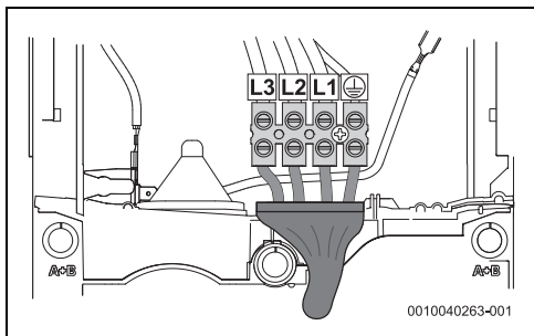
Fig. 49 Lower connection short cables
