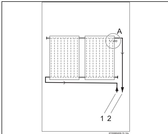
Fig. 45 Mounting location for the collector probe (schematic view)
