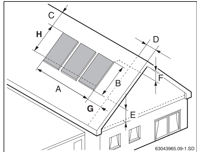
Fig. 6 Dimensions to be maintained
