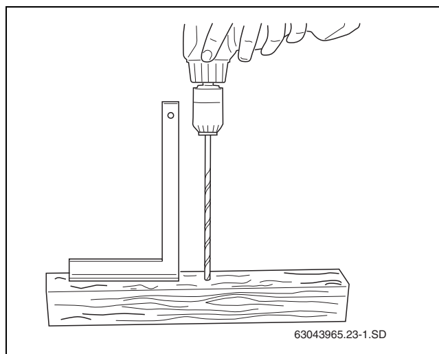
Fig. 21 Creating a drilling template
