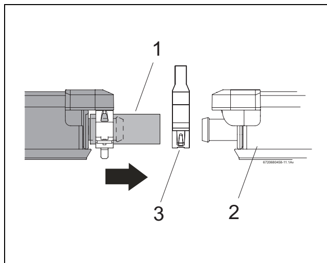
Fig. 41 Pushing the second collector towards the first
