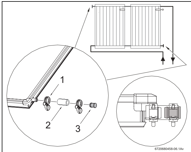
Fig. 35 Assemble the dummy plug and the hose clip
