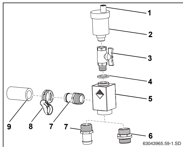
Fig. 50 Standard purge set
