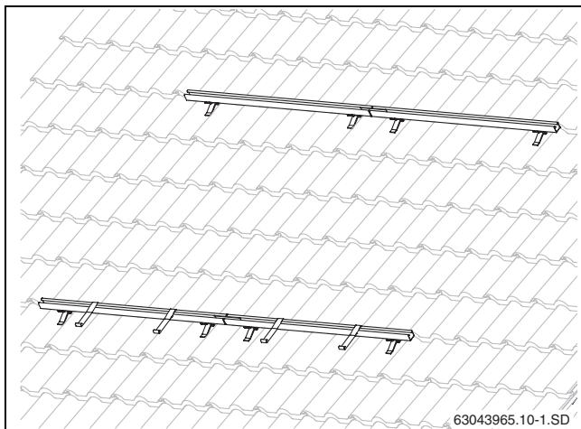
Fig. 7 Pre-assembled profile rails for two collectors
