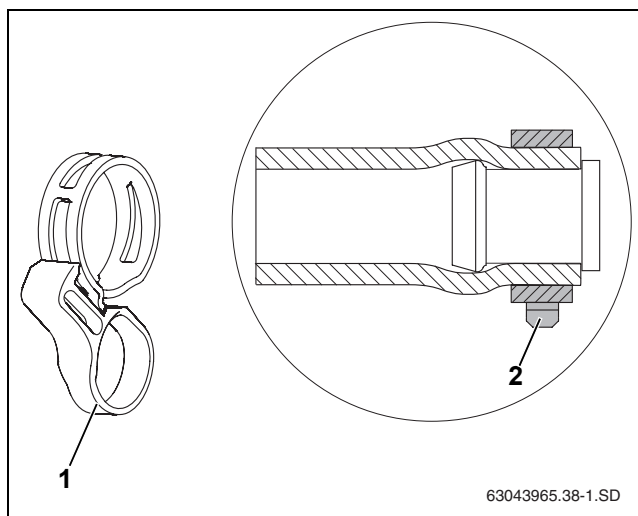
Fig. 32 Hose clip with locking ring fixed to the pre-assembled dummy plug
