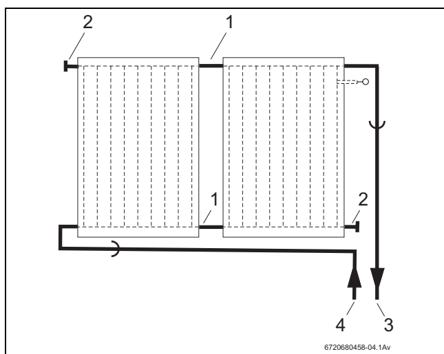
Fig. 33 Hydraulic connection – flow line on the right
