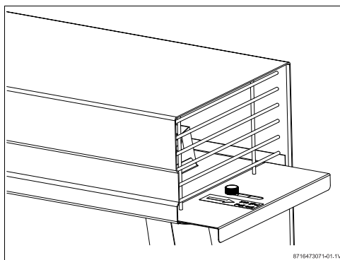
Fig. 6 Flue baffle setting
