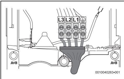
Fig. 51 Lower connection short cables
