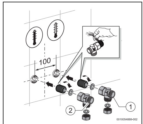
Fig. 16 Horizontal water connections
