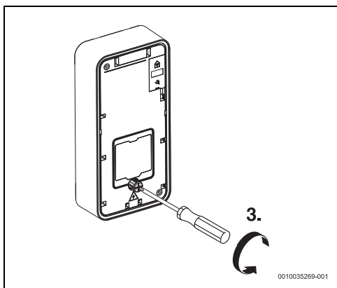
Fig. 11 Loosen the screw
