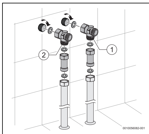
Fig. 17 Vertical water connections
