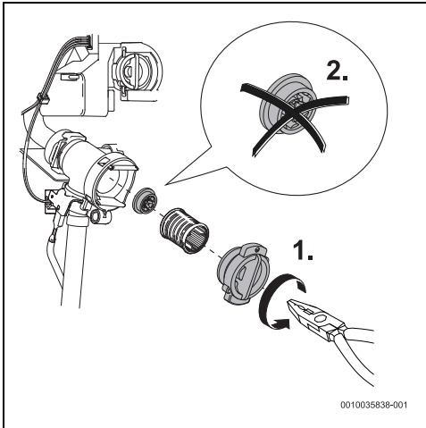
Fig. 56 Remove the flow limiter
